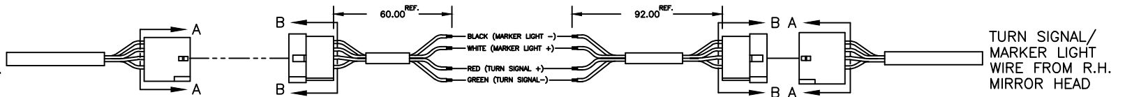
TURN SIGNAL/MARKER LIGHT WIRE HARNESS #747019
